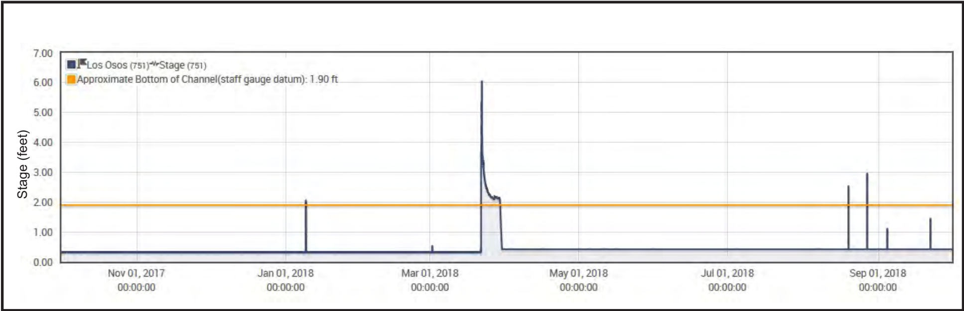
Figure I8 Stream Stage for 2018 Water Year Los Osos Creek, Gage #751
