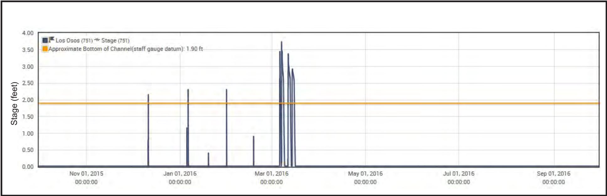
Figure I6 Stream Stage for 2016 Water Year Los Osos Creek, Gage #751
