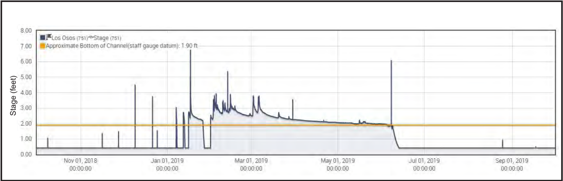
Figure I9 Stream Stage for 2019 Water Year Los Osos Creek, Gage #751
