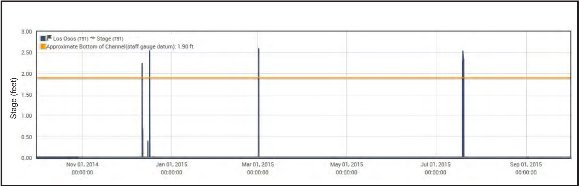
Figure I5 Stream Stage for 2015 Water Year Los Osos Creek, Gage #751
