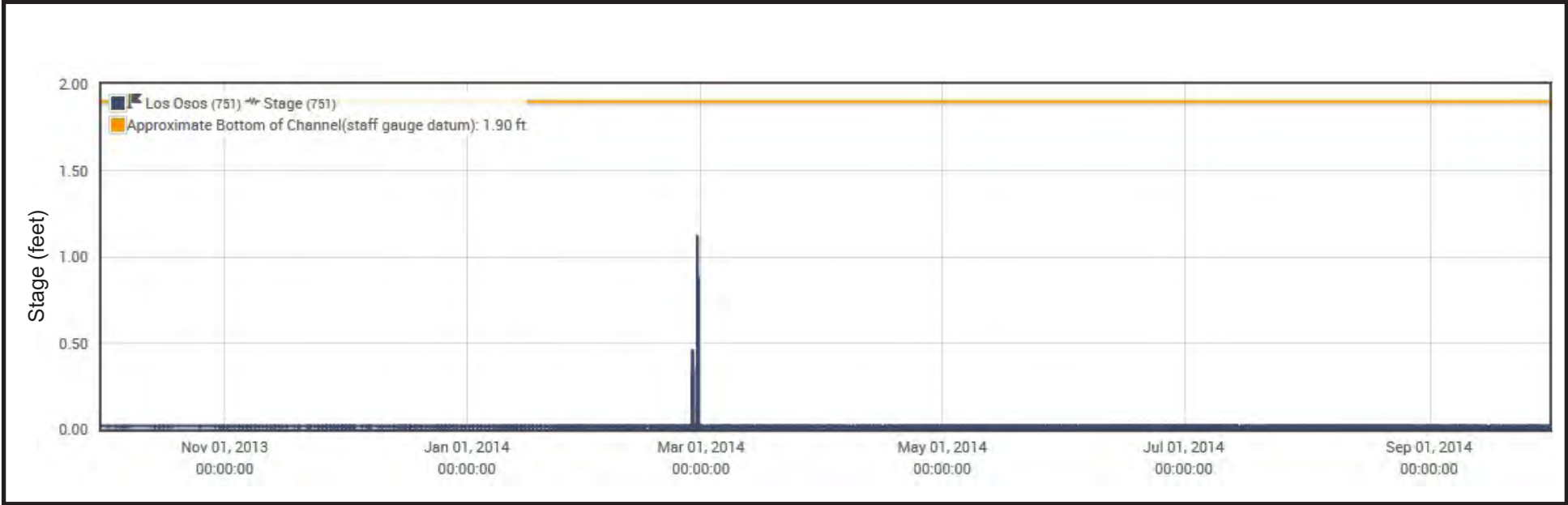
Figure I4 Stream Stage for 2014 Water Year Los Osos Creek, Gage #751
